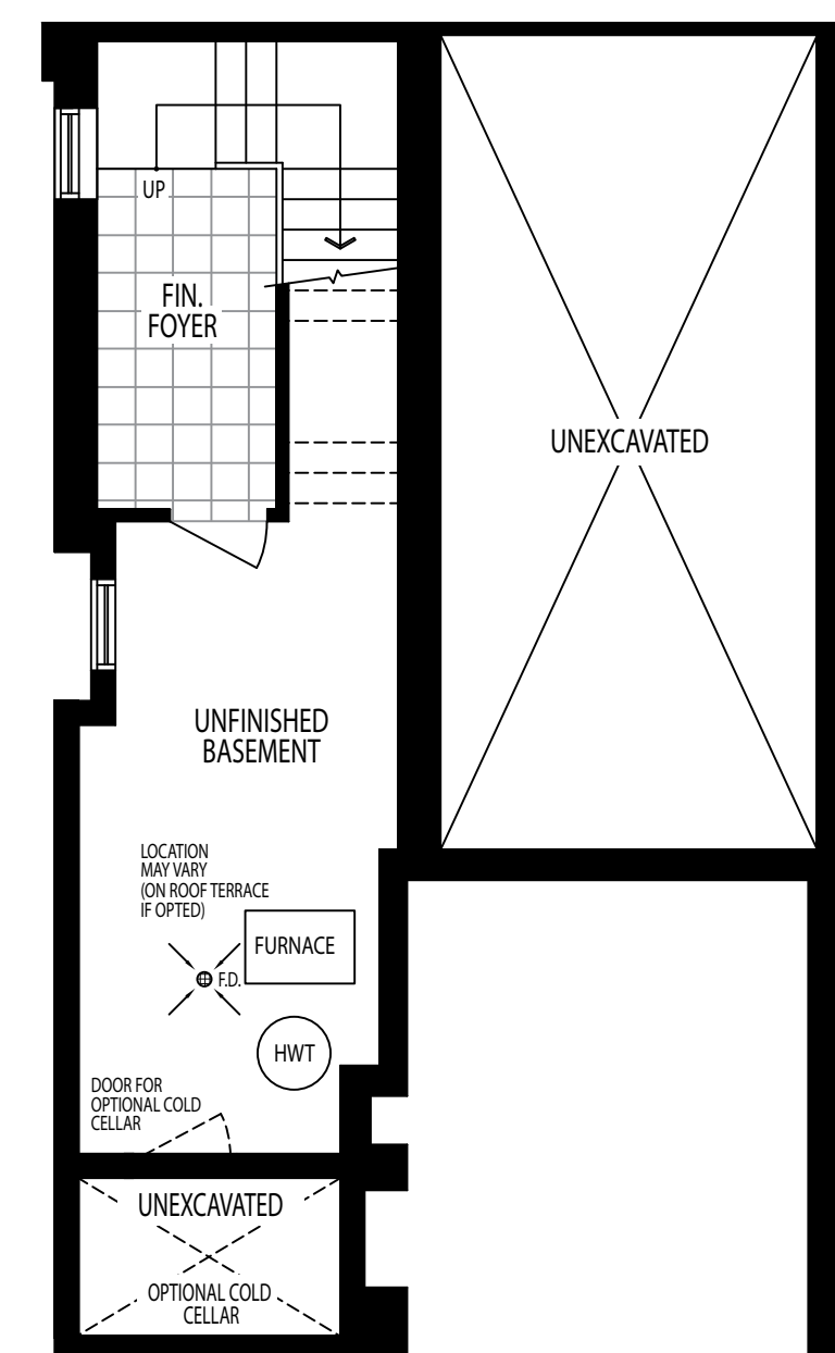
BASEMENT PLAN END UPGRADE ELEV. A
