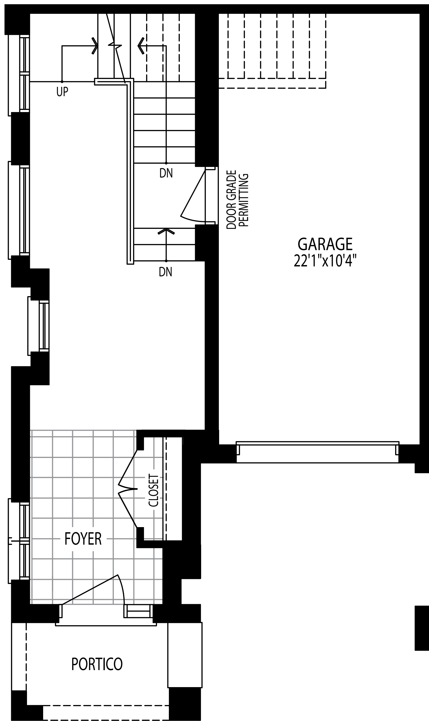
GROUND FLOOR PLAN END UPGRADE ELEV. A
