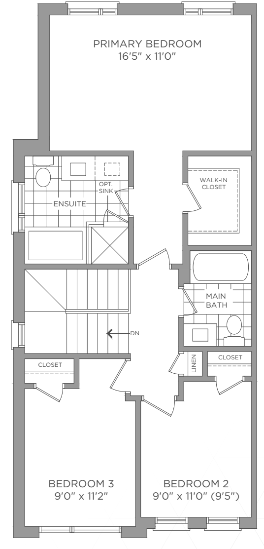
THIRD FLOOR ELEVATION A
