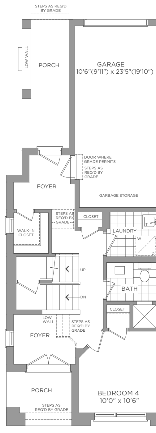
OPT. FIRST FLOOR ELEVATION A
